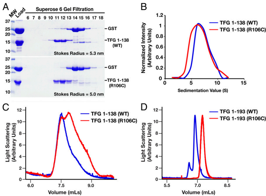
Fig. 2. Mutant p.R106C isoforms of TFG exhibit defects in normal oligomerization in vitro. (A) Purified GST-fused forms of WT and p.R106C TFG (amino acids 1–138) were cleaved in solution to remove the tag and separated by size-exclusion chromatography. Eluted fractions were separated by SDS/PAGE and stained with Coomassie stain. The Stokes radius of each protein was determined based on the elution profile of characterized standards. (B) Purified proteins described in A were applied to a glycerol density gradient (10–30%) and fractionated by hand. Individual fractions recovered were separated by SDS/PAGE and stained by using Coomassie stain. Densitometry measurements were made to quantify the amount of protein in each fraction, which is presented in a graphical format. (C and D) WT and p.R106C TFG (amino acids 1–138 and 1–193) were purified and examined by light scattering following size-exclusion chromatography. The lack of overlap between the peaks for each pair indicates that the oligomerization of TFG is altered in the presence of the R106C mutation.
